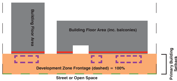
Figure 23: Building Alignment and Articulation – Plan
